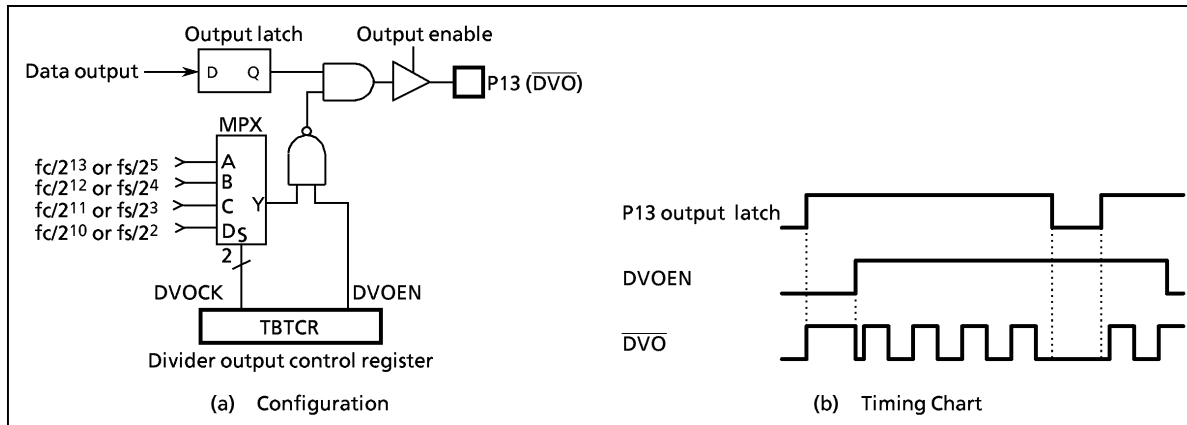
Figure 2-15. Divider Output
