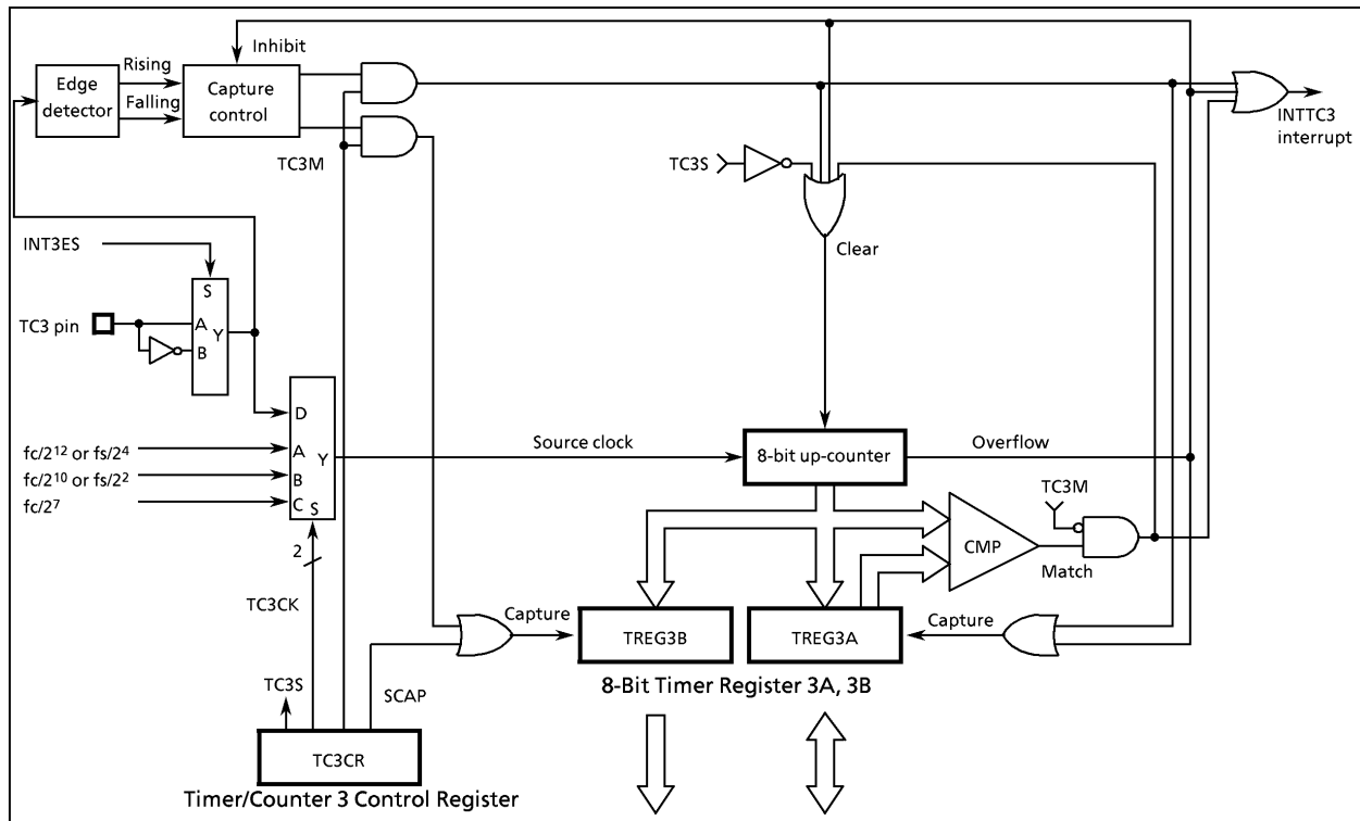
Figure 2-22. Timer/Counter 3
