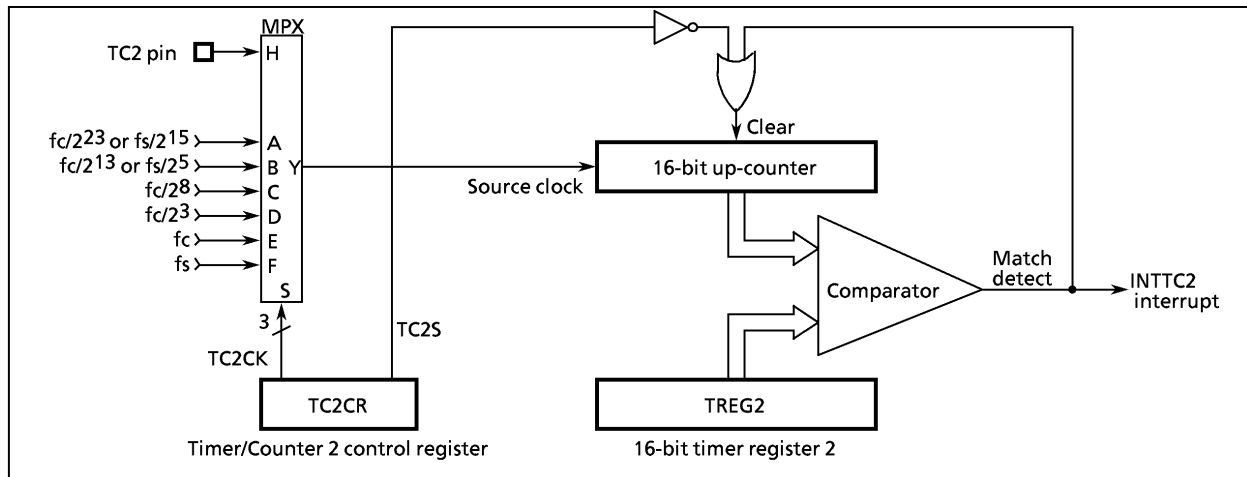
Figure 2-20. Timer/Counter 2
