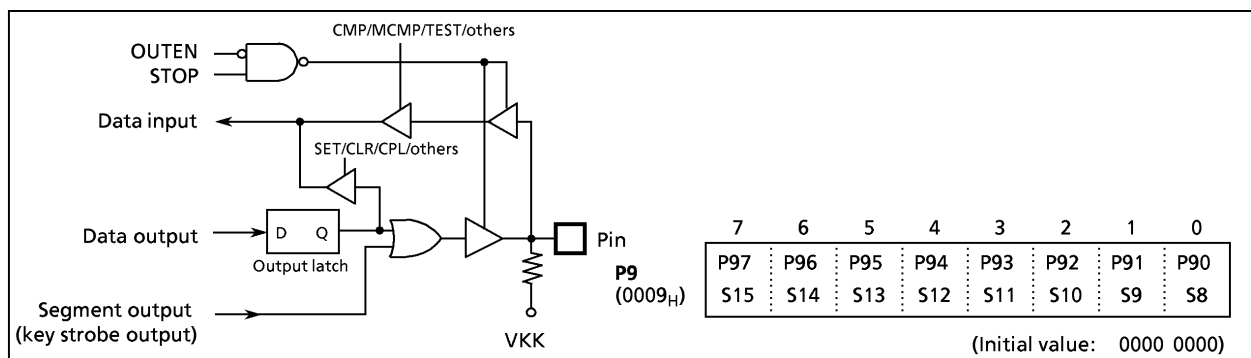
Figure 2-11. Port P9
