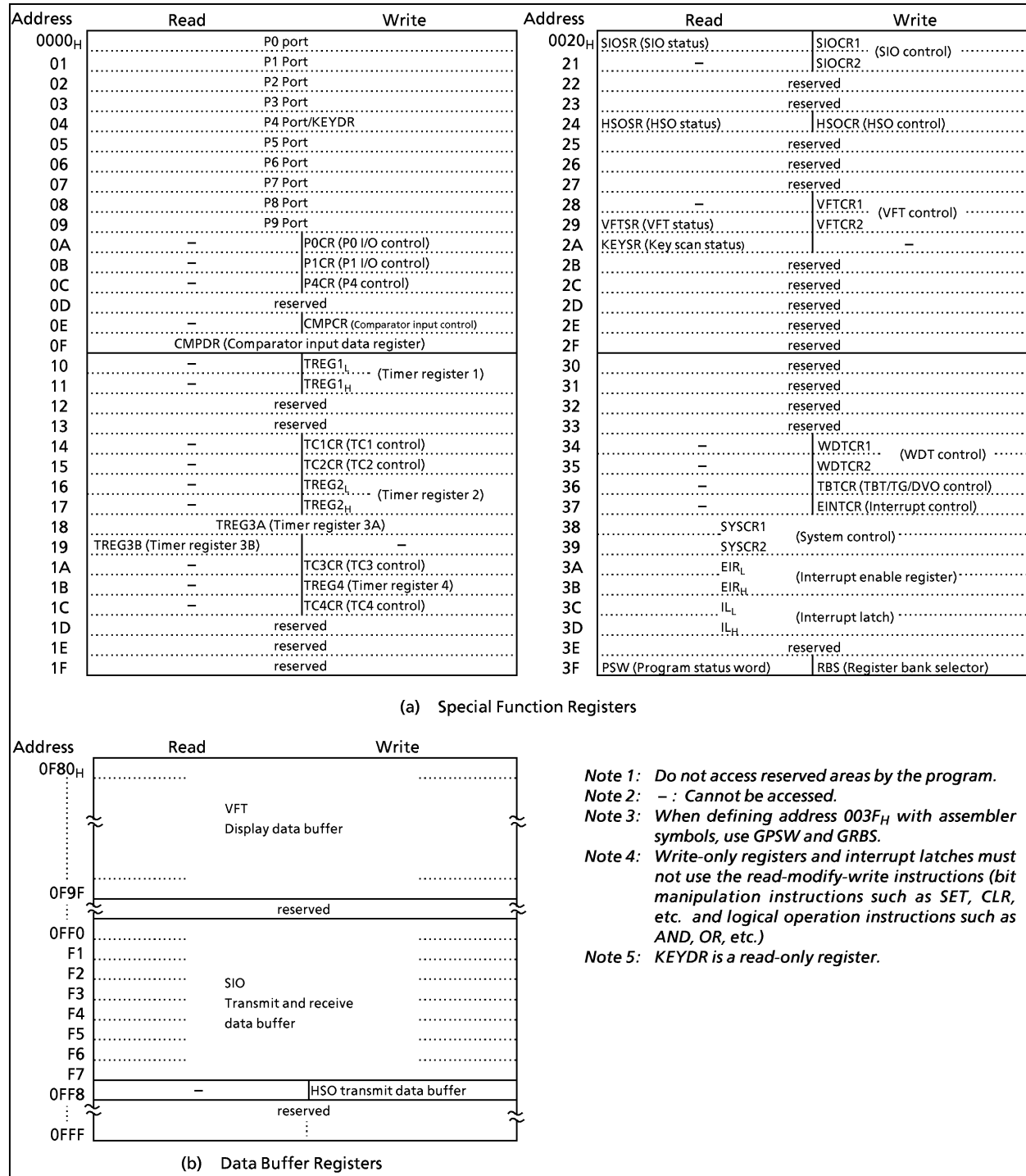
Figure 2-1. SFR & DBR
