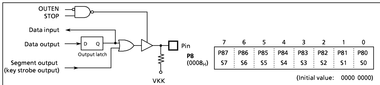
Figure 2-10. Port P8
