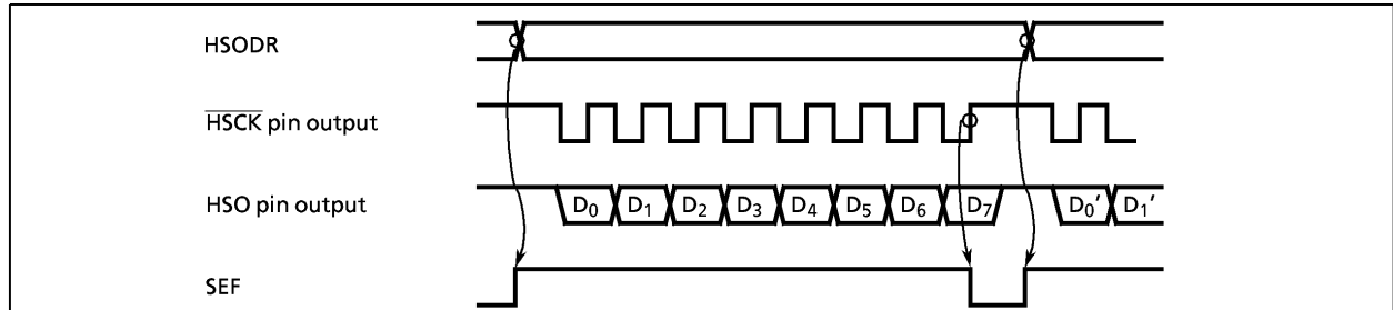
Figure 2-40. High-speed Serial Output Timing Chart
