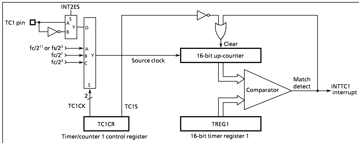
Figure 2-16. Timer/Counter 1
