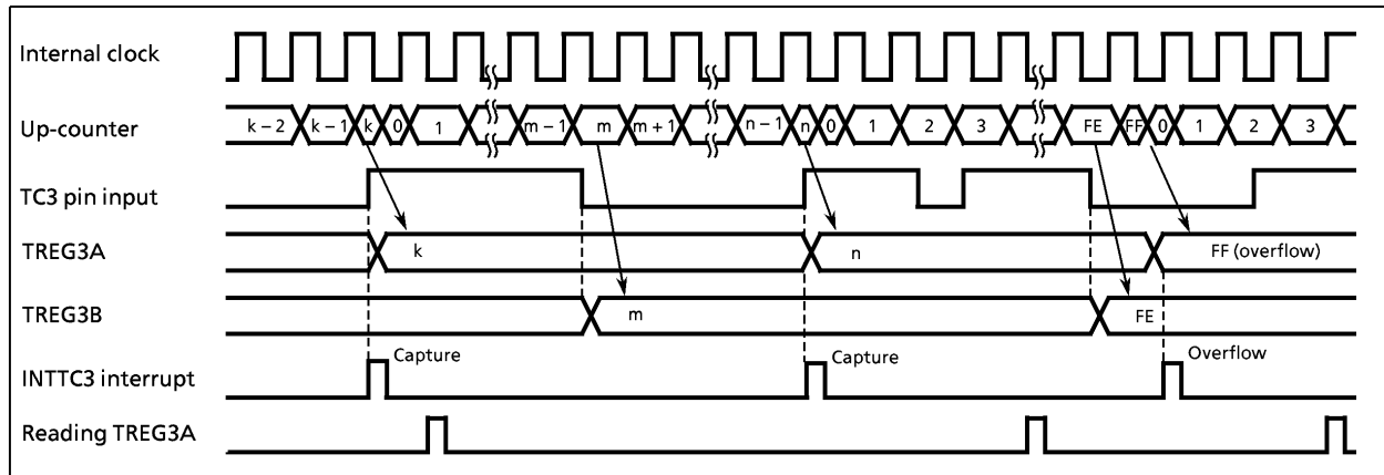
Figure 2-24. Timing Chart for Capture Mode (INT3ES = 0)
