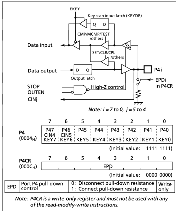
Figure 2-7. Port P4
