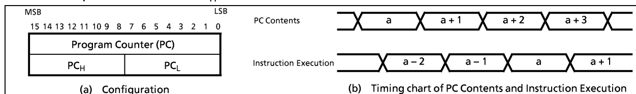
Figure 1-3. Program Counter
