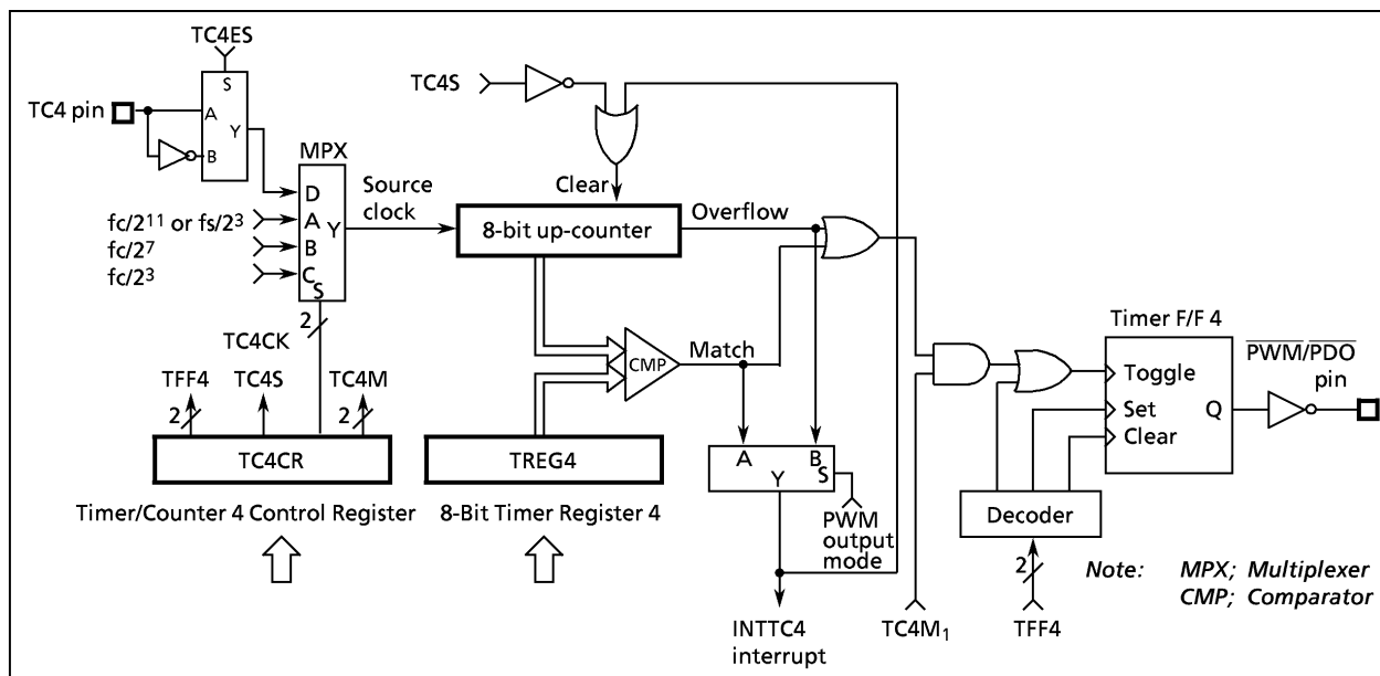
Figure 2-25. Timer/Counter 4
